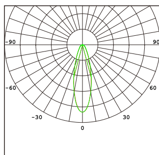
Symmetrical 30° F01604
