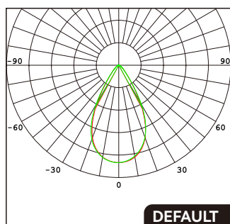
Symmetrical 60° F01605
