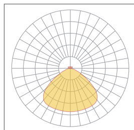
Symmetrical 115° H00200+H00219
