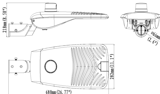
With Photocell
